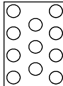
FIGURE 33. VIA PATTERN OF ISL97694A TQFN
