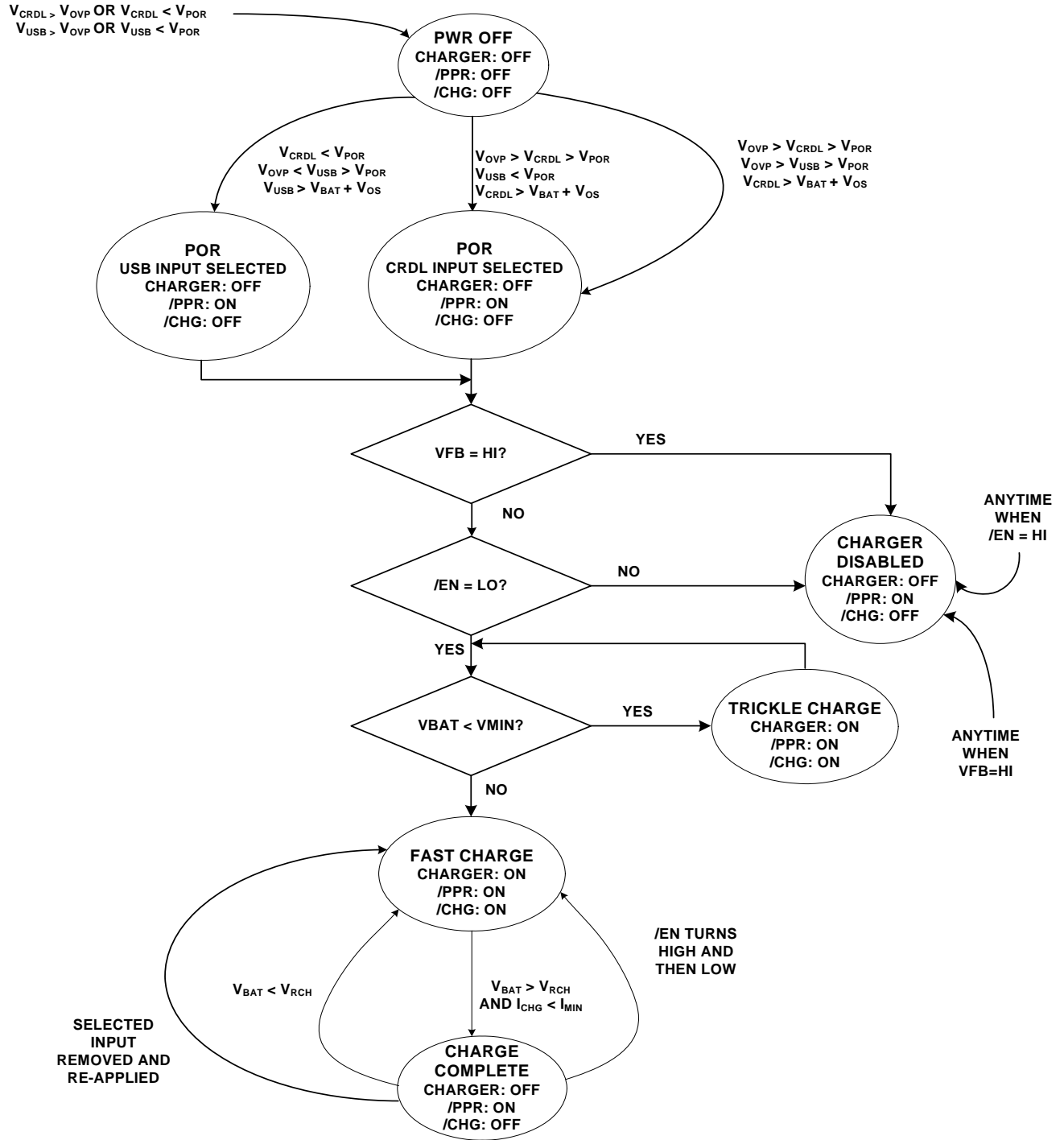
FIGURE 12. STATE DIAGRAM
