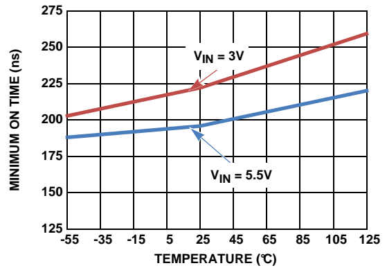
FIGURE 8. LXx MINIMUM ON TIME vs V IN
