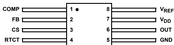
ISL78840ASEH, ISL78841ASEH, ISL78843ASEH, ISL78845ASEH (8 LD FLATPACK) TOP VIEW
