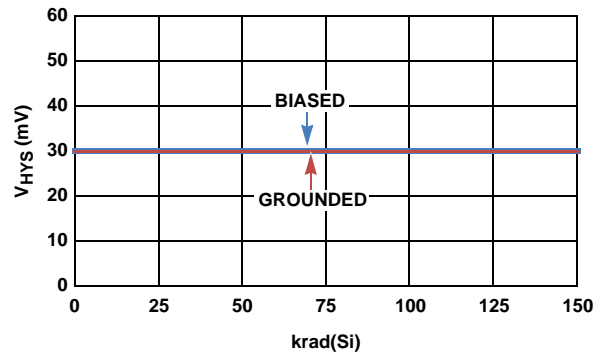
FIGURE 25. ISL706xEH V_{HYS} vs LOW DOSE RATE RADIATION
