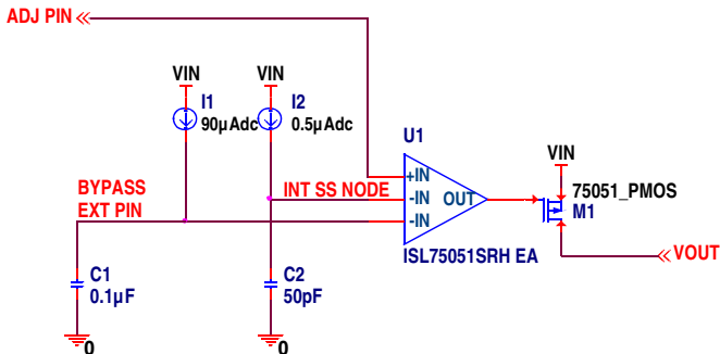
FIGURE 23. SOFT-START
