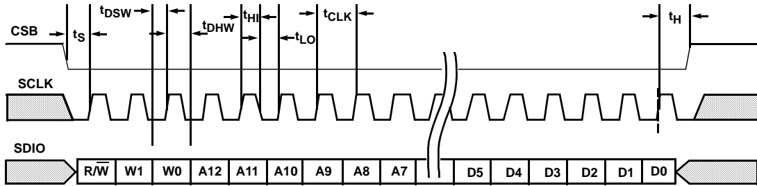
FIGURE 37. SPI WRITE
