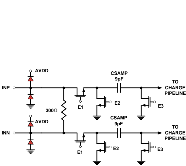
FIGURE 42. ANALOG INPUTS
