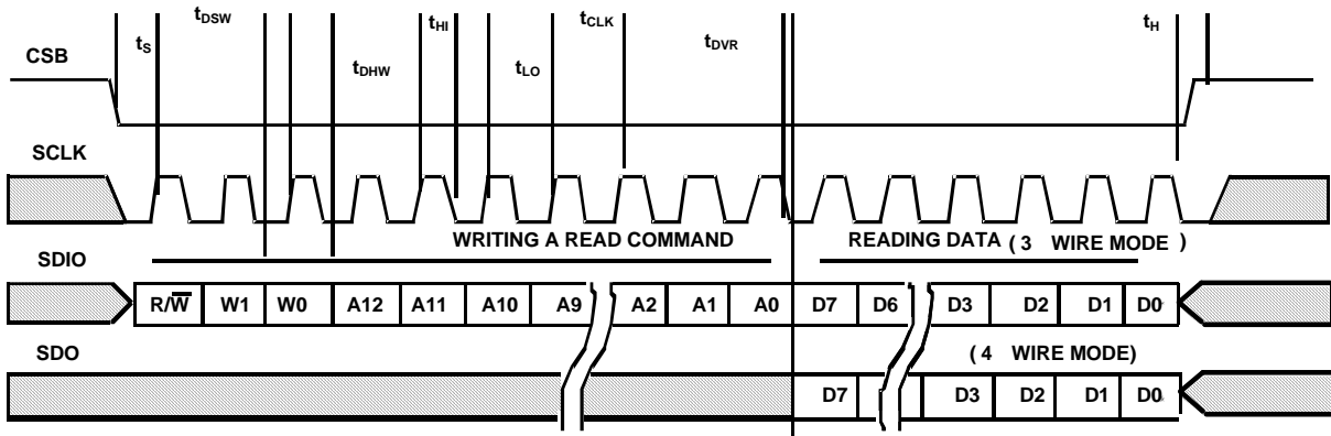
FIGURE 38. SPI READ
