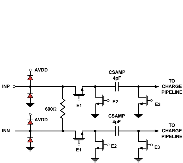
FIGURE 48. ANALOG INPUTS
