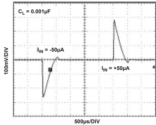
FIGURE 24. 50µA LOAD TRANSIENT RESPONSE
