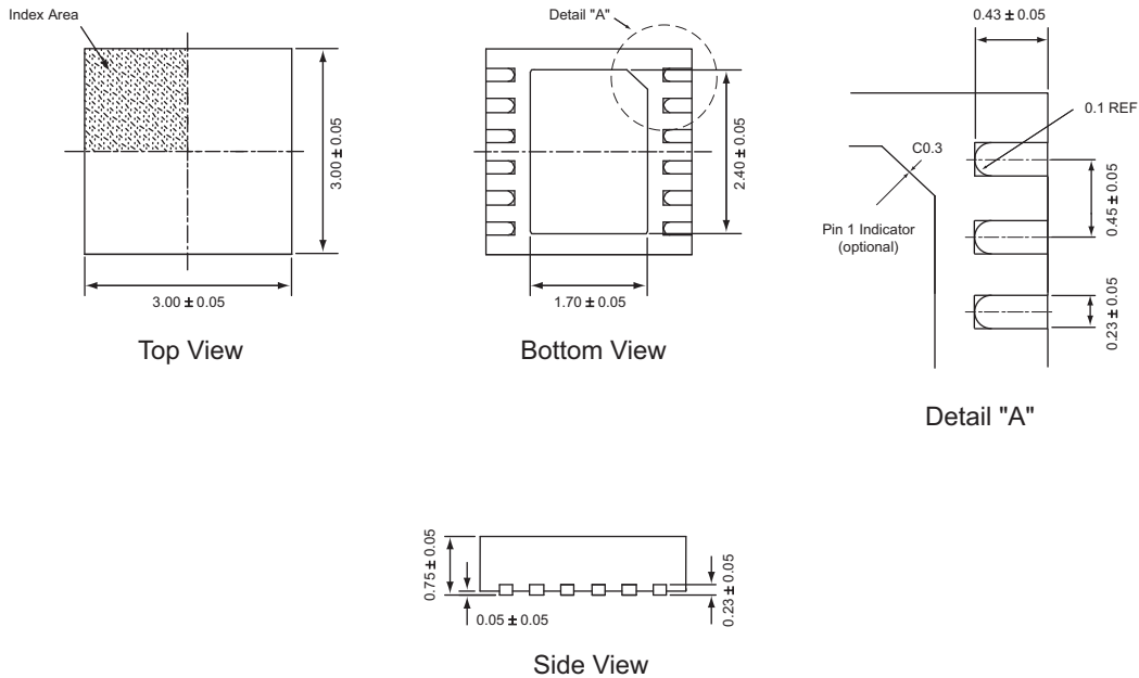
TDFN33-12 3
