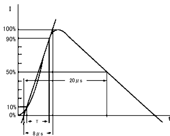
Fig. 9.2 Based on IEC61000-4-5 8/20 \mu\text{s} pulse.
