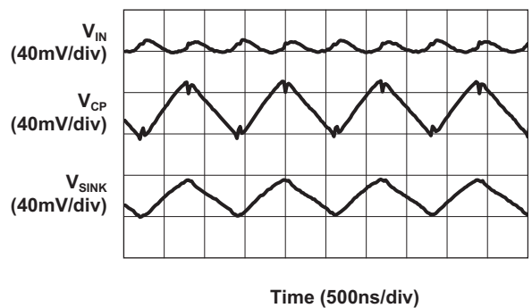
Load Characteristics ( V_{IN} = 2.9\text{V} ; 2X Mode; 14mA Load)
