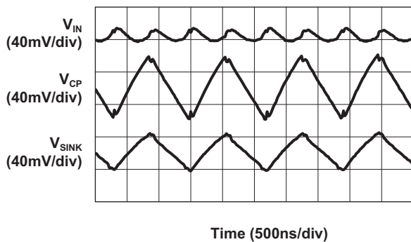
Load Characteristics ( V_{IN} = 2.9\text{V} ; 2X Mode; 20mA Load)
