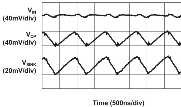
Load Characteristics ( V_{IN} = 3.9\text{V} ; 1.5X Mode; 20mA Load)
