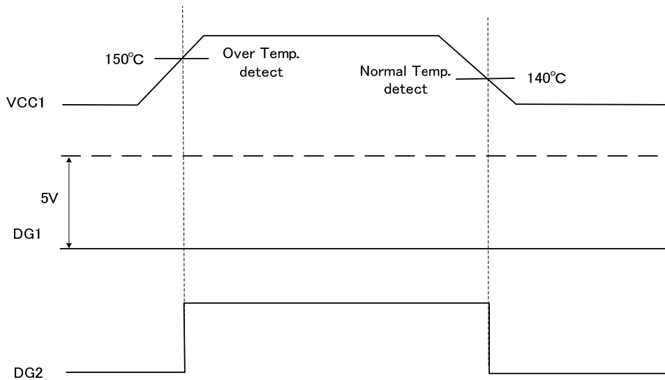
The above is the case to detect only Over Temperature (DG1=L,DG2=H)
