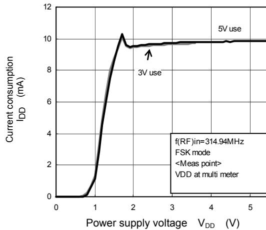
FSK Current Consumption vs. Power Supply Voltage Characteristics
