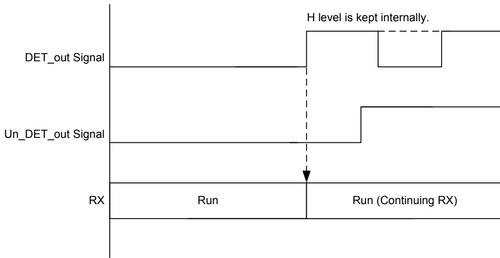
Fig 6-33 AutoOff Type A (Continuing RX)
