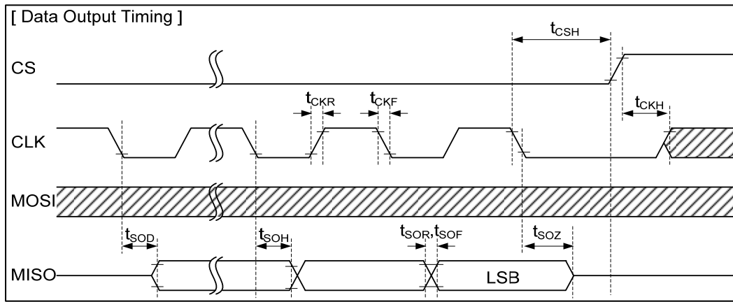
Fig 6-20 Example of SPI Read Timing (Single Read/Write)
