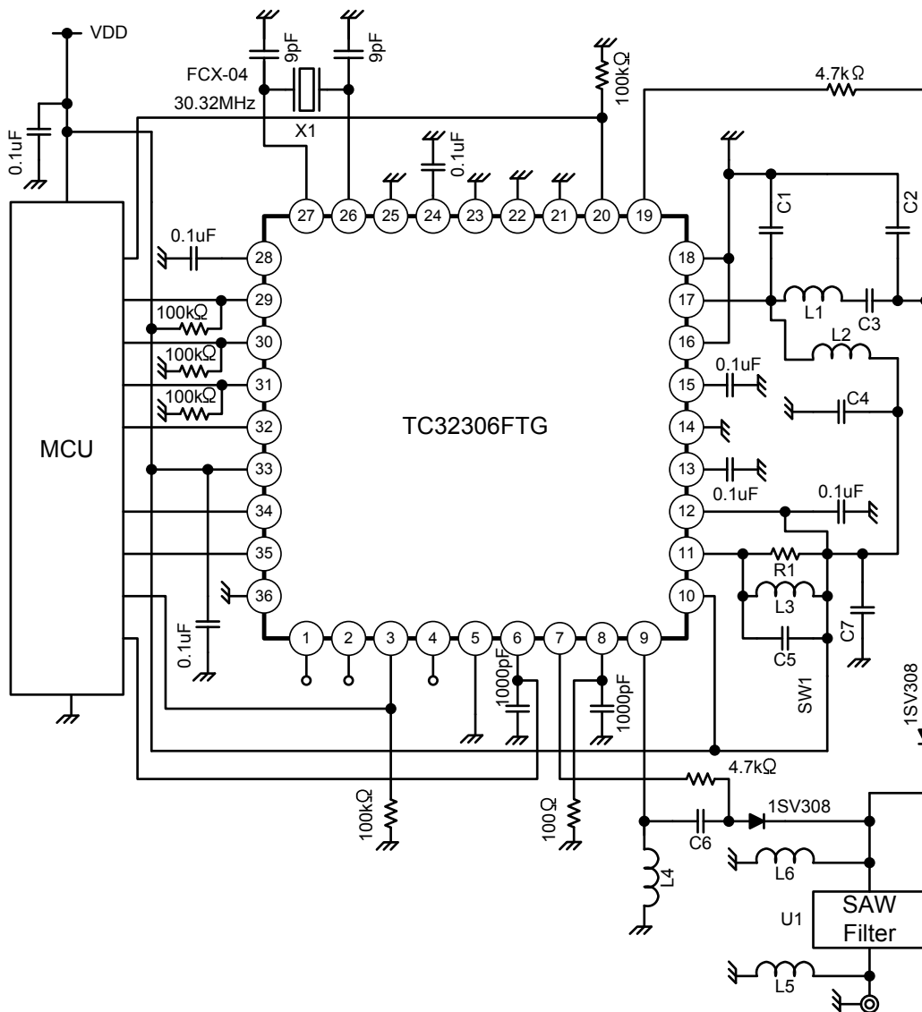
Fig 13-2 Example of Application Circuit 1
