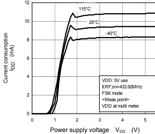
FSK Current Consumption vs. Power Supply Voltage Characteristics 433.92MHz
