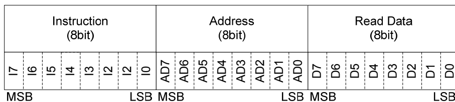
Fig 6-13 SPI Control Data Format
