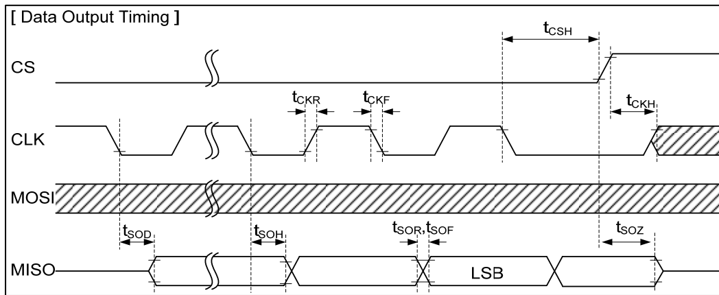
Fig 6-21 Example of SPI Read Timing (Burst Read/Write)
