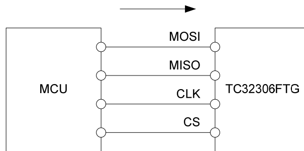
Fig 6-12 Conceptual Connection of SPI Control
