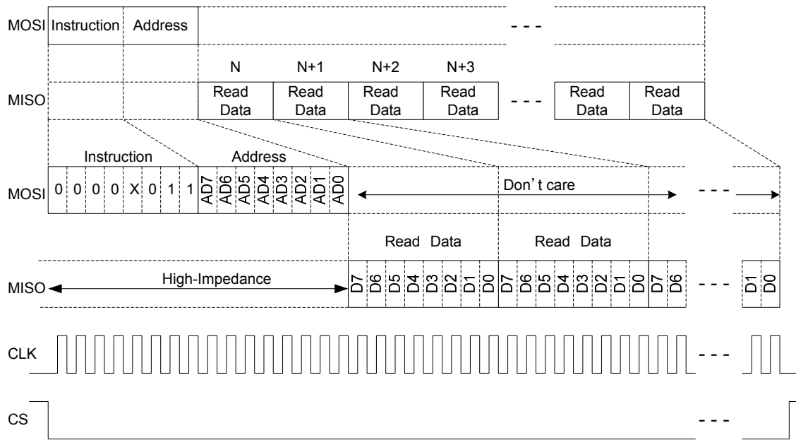
Fig 6-17 Read Format (SPI Burst Read/Write)
