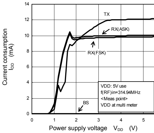
RX Current Consumption vs. Power Supply Voltage Characteristics
