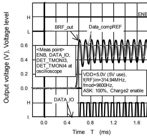
Data Comparator, Response Characteristics of Rise Time ASK (bit rate = 9600Hz)
