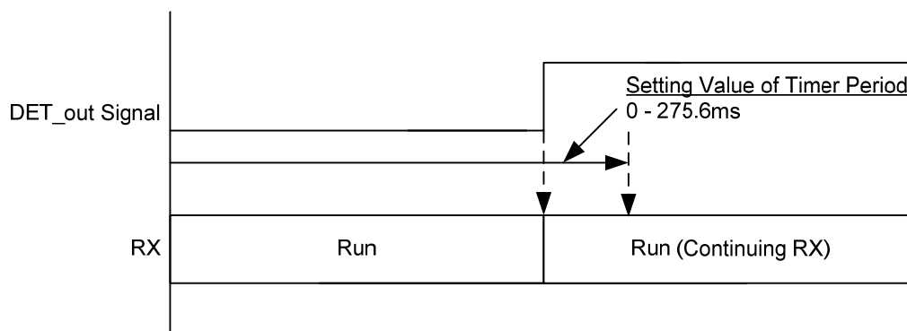
Fig 6-35 AutoOff Type B (Continuing RX)
