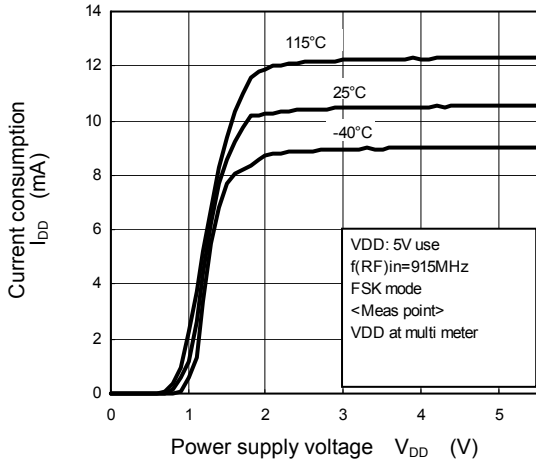
FSK Current Consumption vs. Power Supply Voltage Characteristics 915MHz
