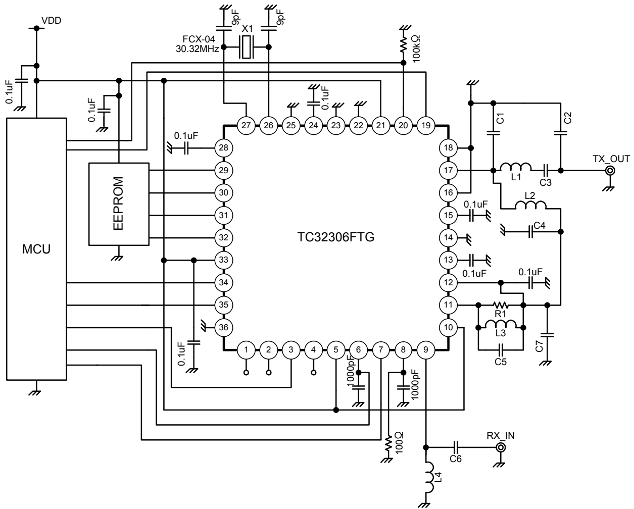
Fig 13-3 Example of Application Circuit 2
