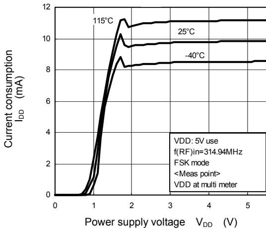
FSK Current Consumption vs. Power Supply Voltage Characteristics 314.94MHz
