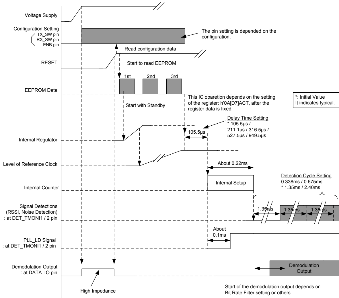
Fig 6-30 Example of Boot Sequence Timing Chart (EEPROM Mode / RX)
