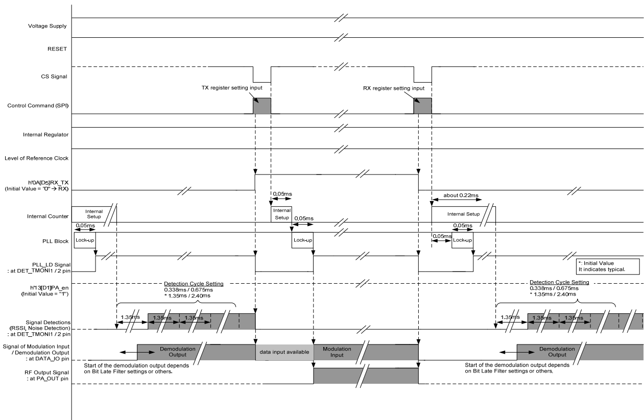
Fig 6-31 Example of Timing Chart (RX → TX → RX in SPI Mode)
