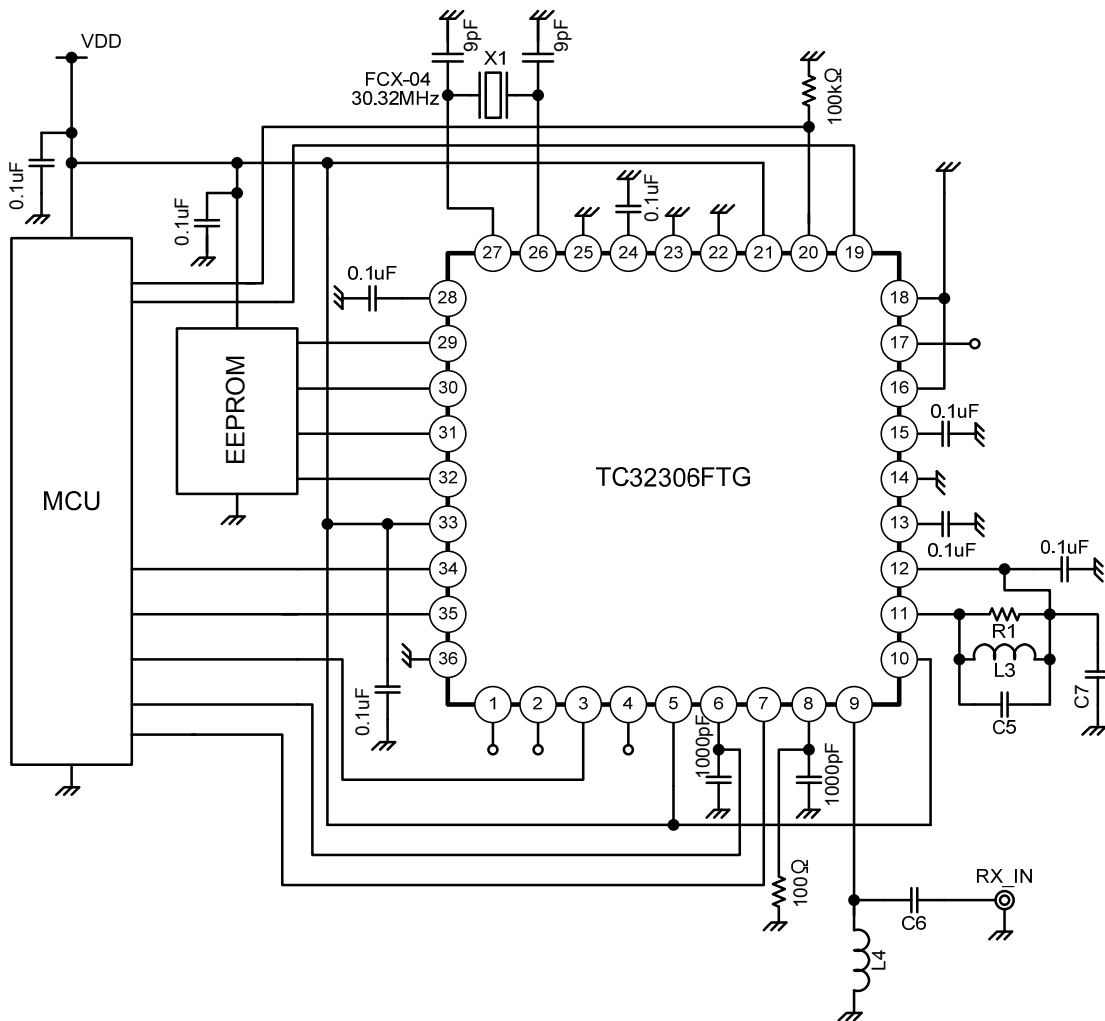
Fig 13-4 Example of Application Circuit 3
