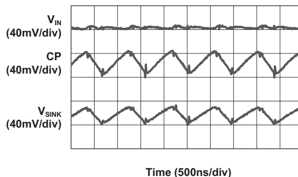
Load Characteristics ( V_{IN} = 3.9V ; 1.5X Mode; 20mA Load)
