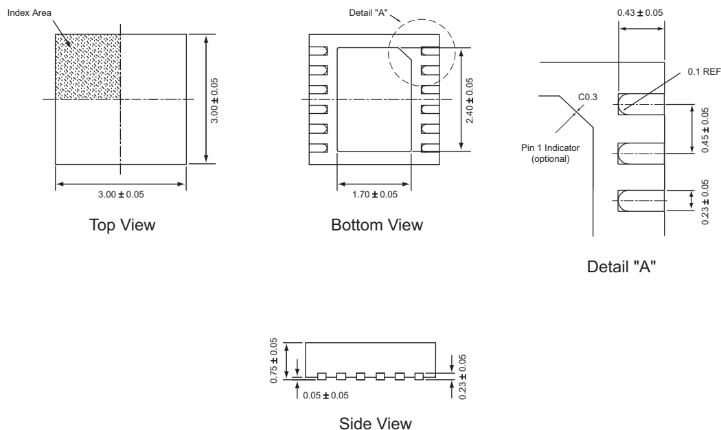
TDFN33-12
