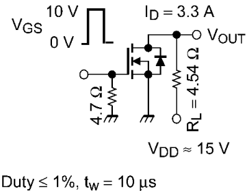
Fig. 6.2.1 Switching Time Test Circuit (P-ch) Fig. 6.2.2 Switching Time Test Circuit (N-ch)
