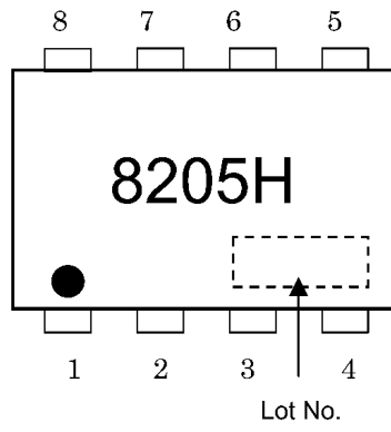
Fig. 7.1 Marking
