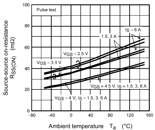
Fig. 10.6 R_{SS(ON)} - T_a (Note 6)
