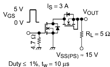
Fig. 7.2.1 Switching Time Test Circuit
