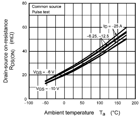
Fig. 8.6 R_{DS(ON)} - T_a (Note 8)
