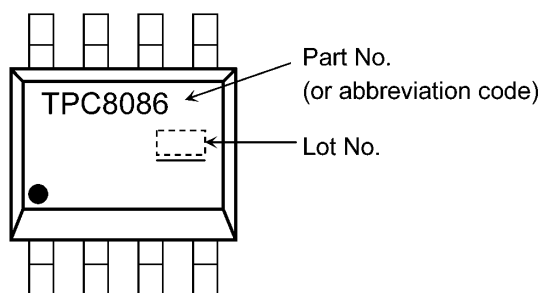
Fig. 7.1 Marking
