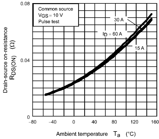
Fig. 8.7 R_{DS(ON)} - T_a
