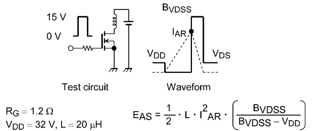
Fig. 8.15 Test Circuit/Waveform
