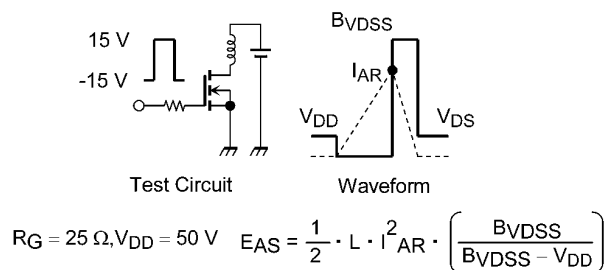
Fig. 8.16 Test Circuit/Waveform
