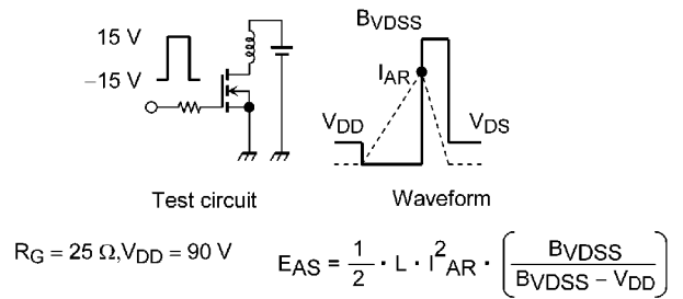
Fig. 8.16 Test Circuit/Waveform
