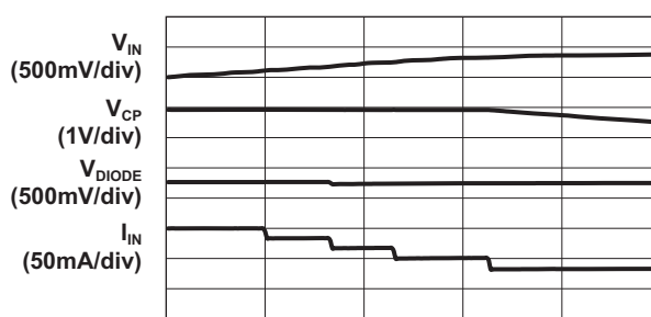
Charge Pump to Load Switch (1.5X Mode, 4x30mA Load)
