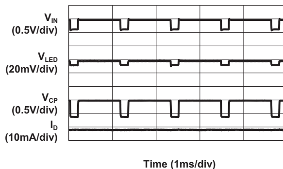
Line Response (1X Mode, 4x30mA Load)
