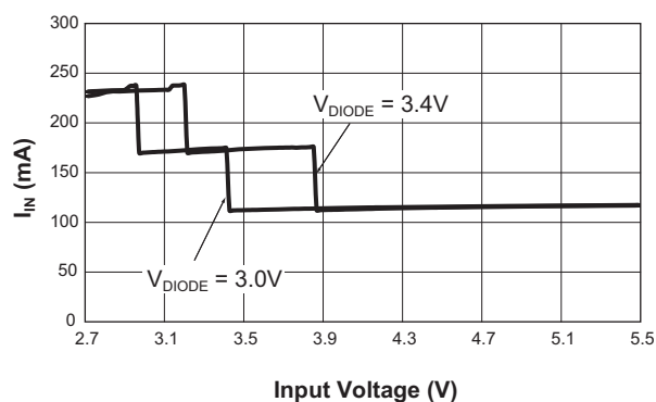
Input Current vs. Input Voltage (4x30mA)
