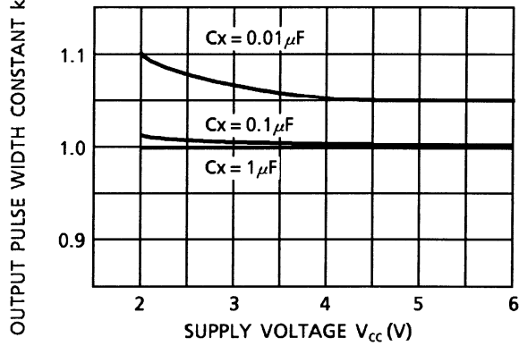
Output Pulse Width Constant K – Supply Voltage (typical) (EXTERNAL RESISTOR ( R_x ) = 10\text{k}\Omega : t_{WOUT} = K \cdot C_x \cdot R_x )
