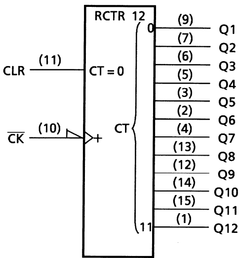
TC74HC4040A
