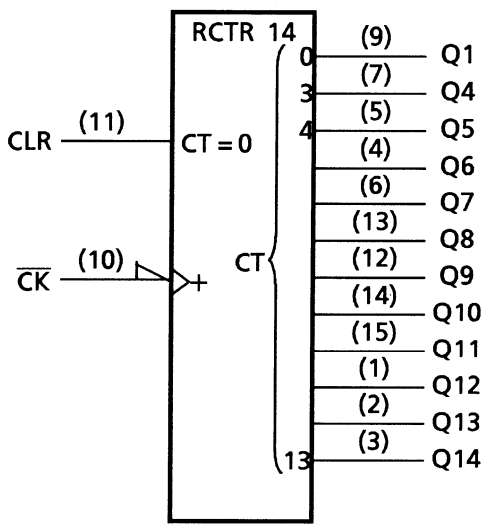
TC74HC4020A
