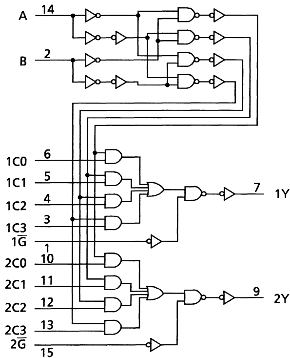
TC74HC153A
