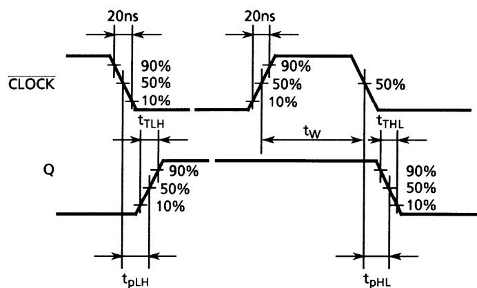
Waveform 1
