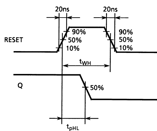
Waveform 2
