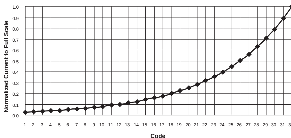
Figure 1: Normalized Current Level Settings.
