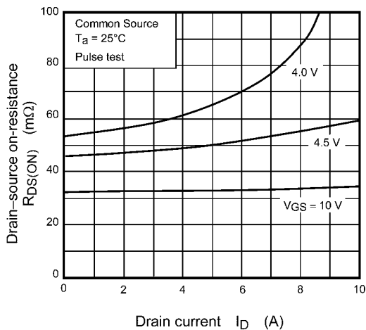
Fig. 7.5 R_{DS(ON)} - I_D
