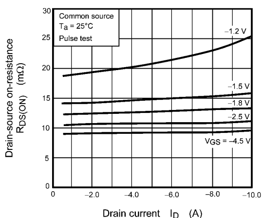
Fig. 7.5 R_{DS(ON)} - I_D
