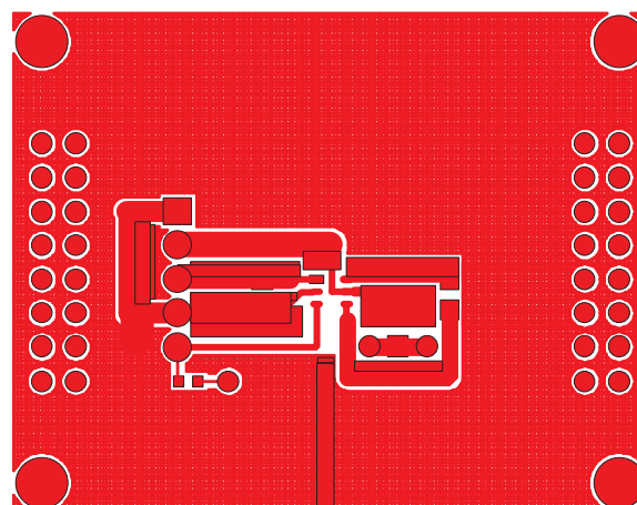
Figure 4: Evaluation Board Component Side Layout.
