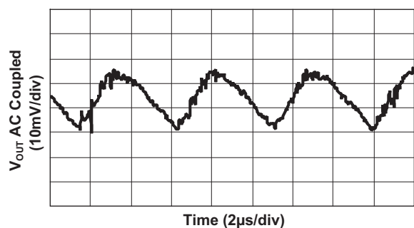
Output Ripple ( I_{OUT} = 50mA ; V_{IN} = 2.5V )
