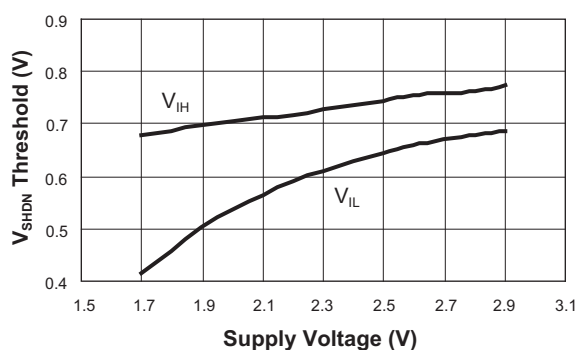
V_{SHDN} Threshold vs. Supply Voltage
