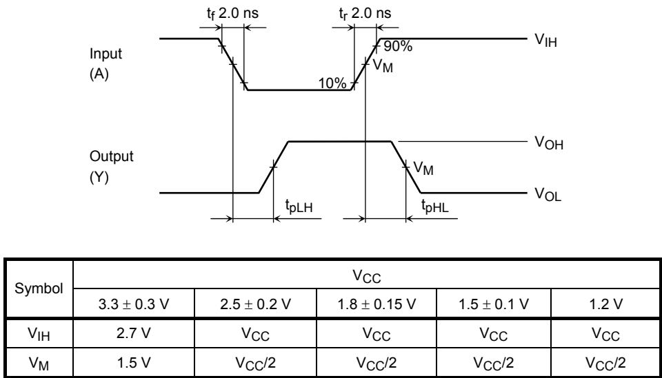
Figure 2 t_{pLH} , t_{pHL}
