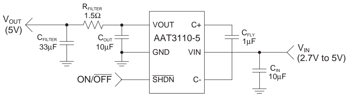
Figure 2: Application With Output Ripple Reduction Filter.
