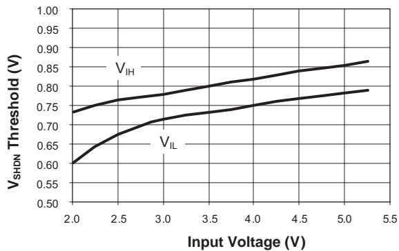
V_{SHDN} Threshold vs. Input Voltage
