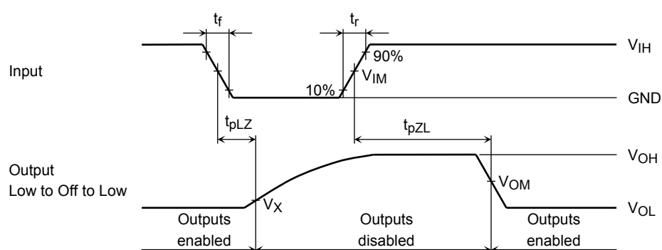
Figure 2 t_{pLZ} , t_{pZL}
