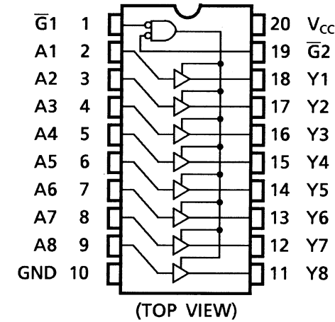
TC74HCT541A
