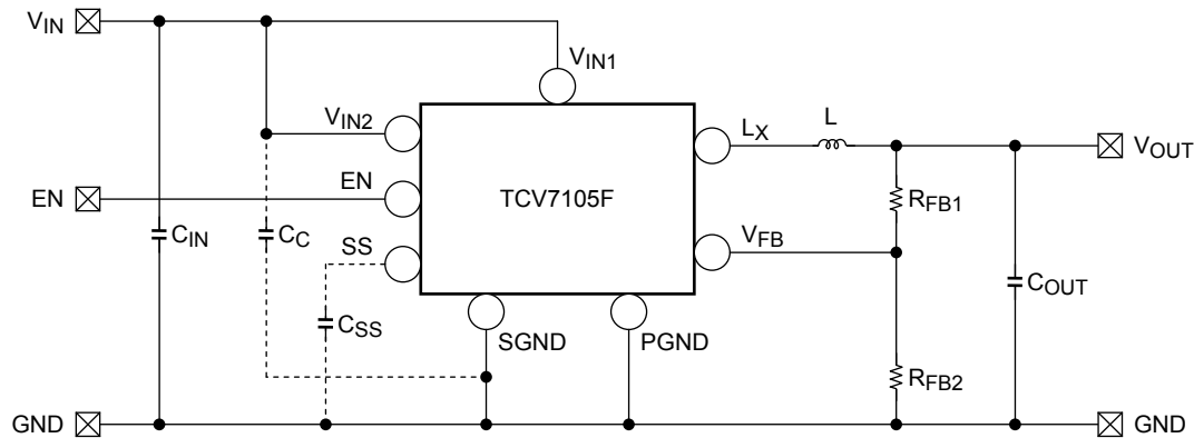
Figure 1 TCV7105F Application Circuit Example
