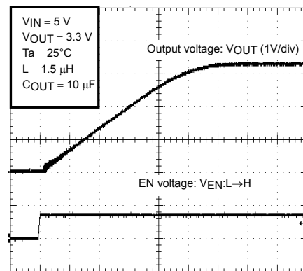
Startup Characteristics ( C_{SS} = 0.1\text{ }\mu\text{F} )
