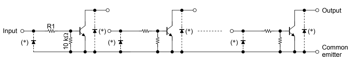
TD62503FNG
