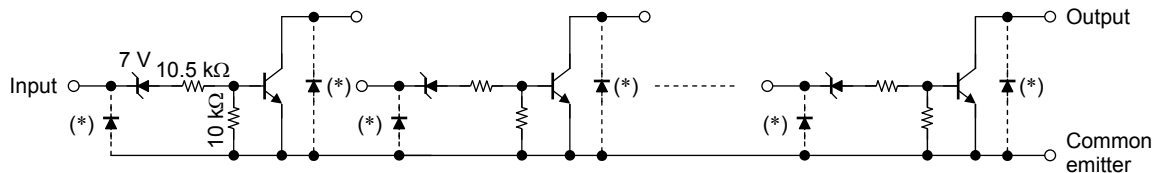
TD62503FNG
