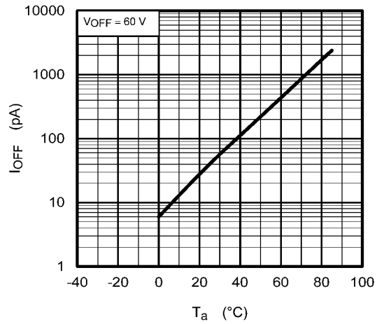
Fig. 13.1.10 I OFF - T a
