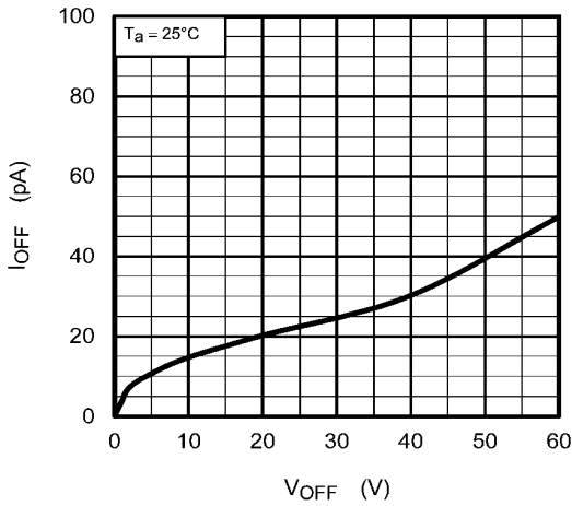
Fig. 13.1.9 I OFF - V OFF
