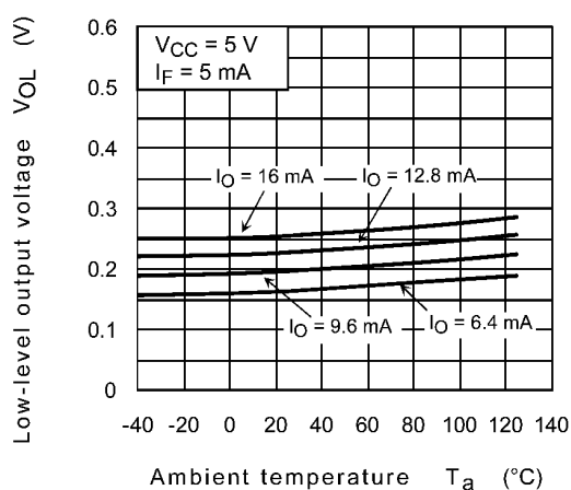
Fig. 12.2.3 V_{OL} - T_a
