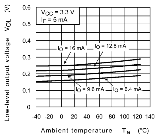
Fig. 12.2.4 V_{OL} - T_a
