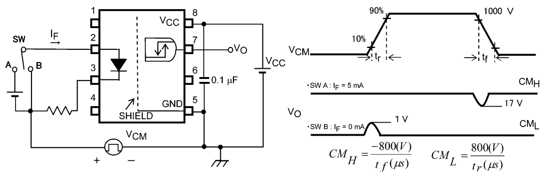
Fig. 12.1.9 Common-Mode Transient Immunity Test Circuit
