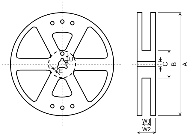
Figure 3 Reel Form
