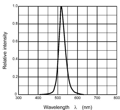
Fig. 8.4 Wavelength Characteristic
