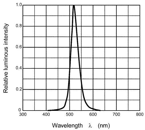
Fig. 8.4 Wavelength Characteristic
