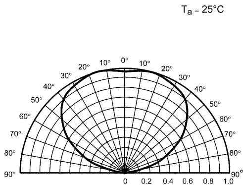
Fig. 8.3 Relative Luminous Intensity - T_a
