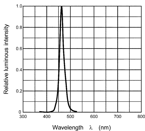
Fig. 8.4 Wavelength Characteristic
