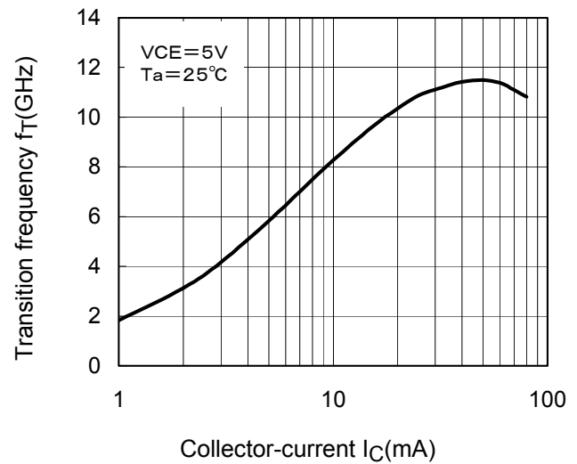
f_T-I_C
