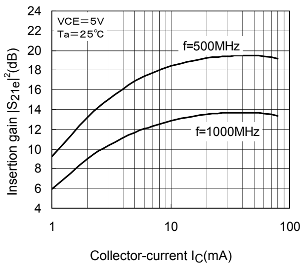
|S_{21e}|^2-I_C
