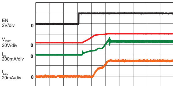
Start Up Waveform
