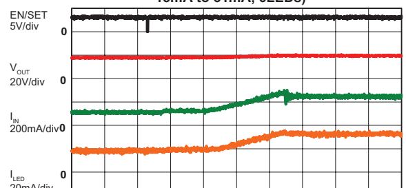
LED Current Transient
