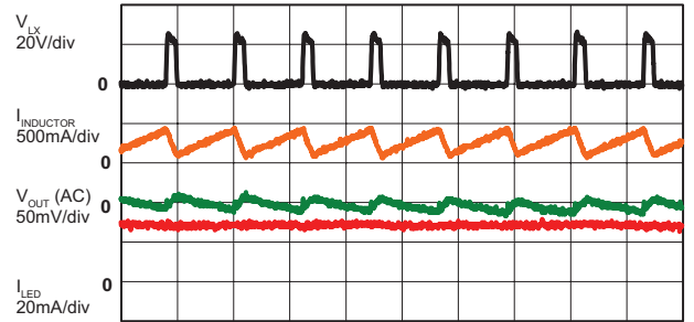
Operation Waveform
