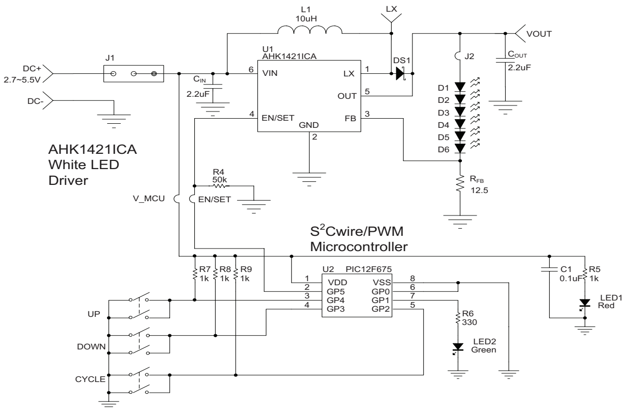
Figure 2: AHK1421 ICA Evaluation Board Schematic.
