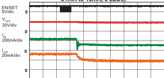
LED Current Transient
