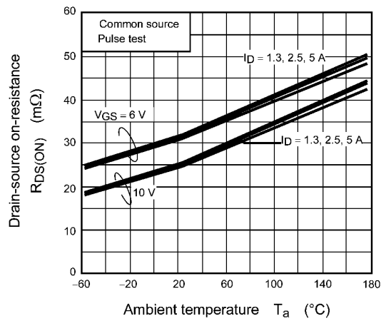
Fig. 8.6 R_{DS(ON)} - T_a (Note 7)
