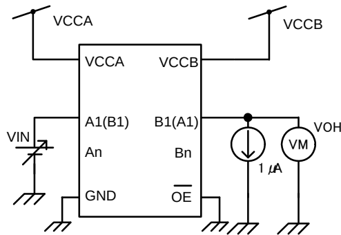
Figure 9 Test Circuit
